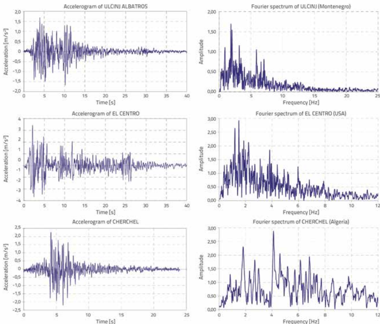
Figure 2. Selected accelerograms and their Fourier spectra
