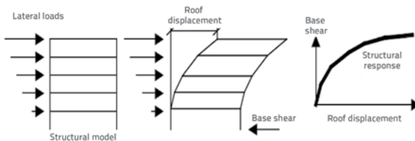
Figure 1. Capacity curve in terms of base shear versus roof displacement
