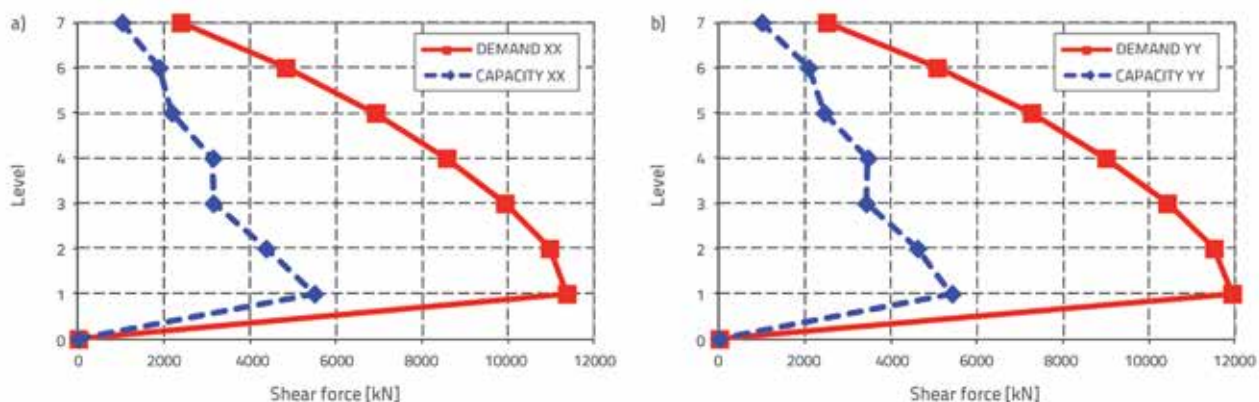
Figure 5. Comparison of capacity and demand in term of shear forces: a) Longitudinal direction; b) Transverse direction
