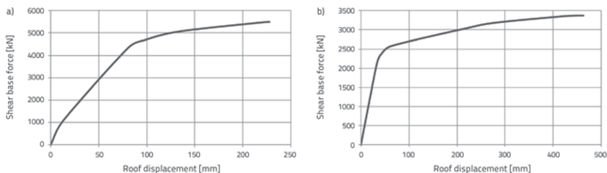
Figure 6. Capacity curves: a) Longitudinal direction; b) Transverse direction
