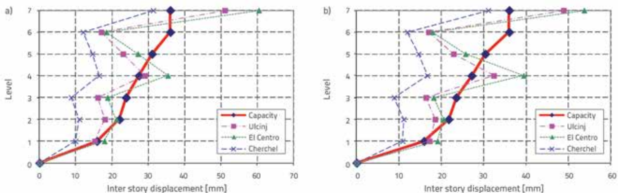
Figure 8. Inter storey displacement by non linear dynamic analysis for both main directions: a) Longitudinal direction; b) Transverse direction
